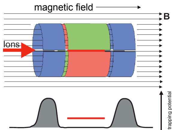
Figure 1-14. Operating principle of the Penning trap
