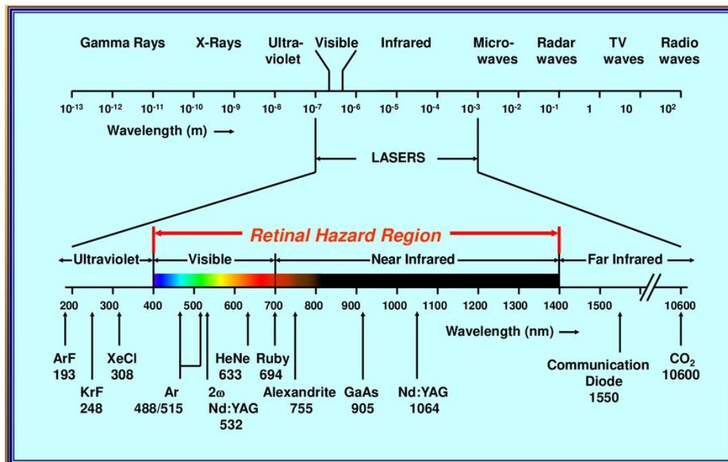
Figure 5 - 1. Retinal Hazard Region (UW-Madison.)
