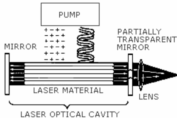
Figure 3 - 1 Simplified Diagram of a Laser
